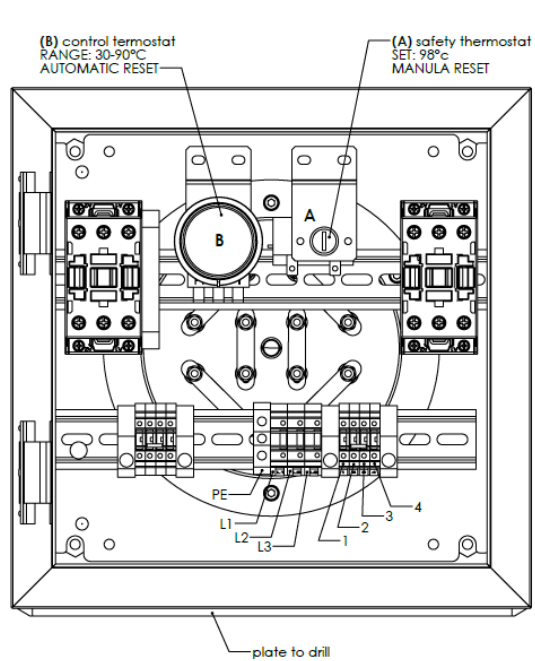
ELECTRICAL DIAGRAM
