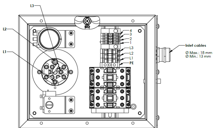
ELECTRIC DIAGRAM
