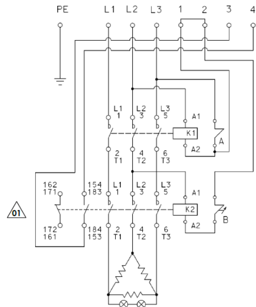
ELECTRICAL DIAGRAM
